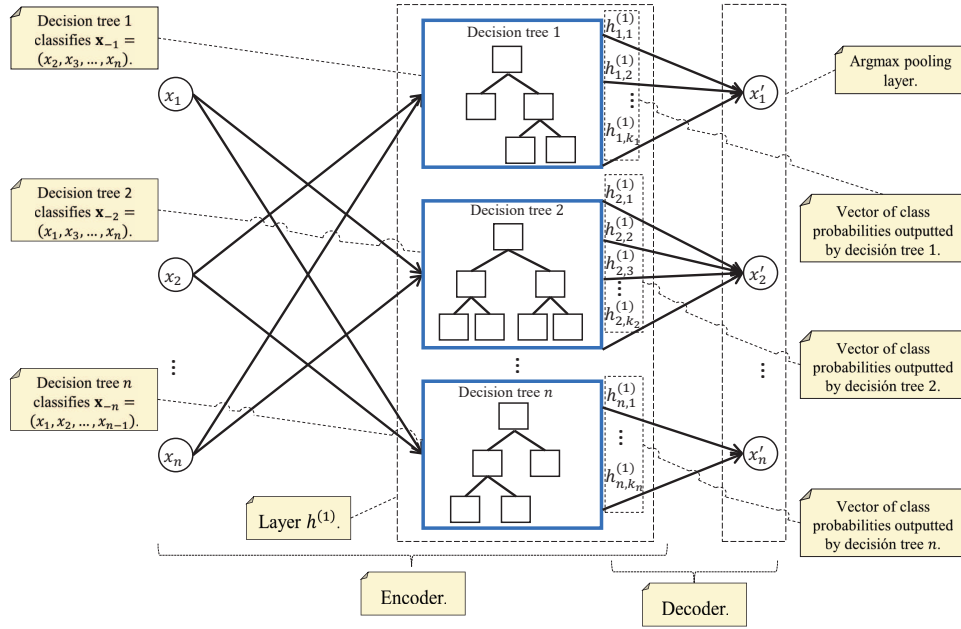
Fig. 2: Architecture of our proposed decision tree-based autoencoder for categorical attributes. In the architecture, the i -th decision tree trains with all the attributes except the i -th attribute. In the classification phase, the i -th decision tree receives a tuple x_{-i} that contains all the attributes values except x_i , and outputs a probability vector which the argmax pooling layer uses to infer x'_i . The length of the i -th vector depends on the number of possible values in the definition domain D_i of the i -th categorical attribute. The end-user can look at the path traversed by the object x_{-i} into the i -th tree, because this path indicates the pattern learned from the training dataset. Hence, the classification result is interpretable.
