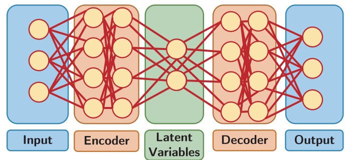
Fig. 1: Autoencoder architecture.
